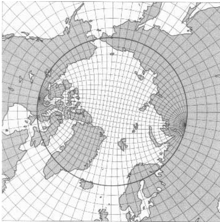
Figure 2: The tripolar grid, often used in ocean modeling. Polar singularities are placed over land and excluded from the simulation.
