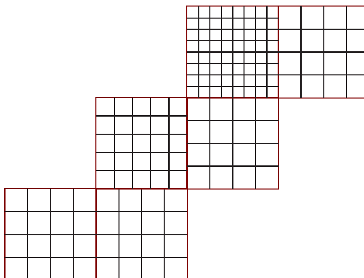
Figure 16: Grid refinement on a cubed-sphere grid mosaic.
