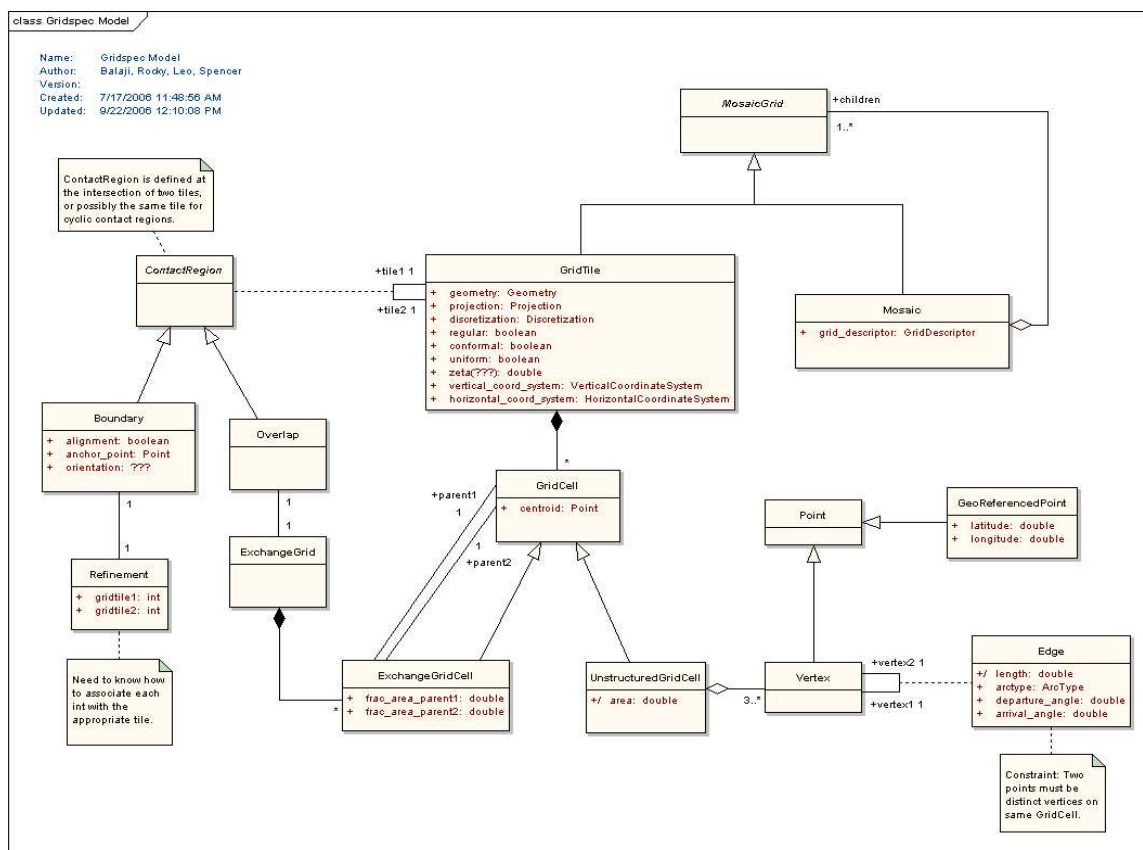
Figure 20: Abstraction of the grid specification. This UML diagram shows schematically how locations, distances, areas and volumes of grid cells are conceptually linked into a structure culminating in a grid mosaic.
