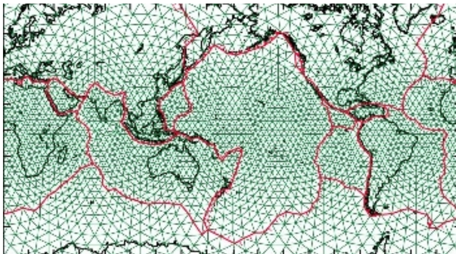
Figure 5: An unstructured triangular discretization of the sphere.
