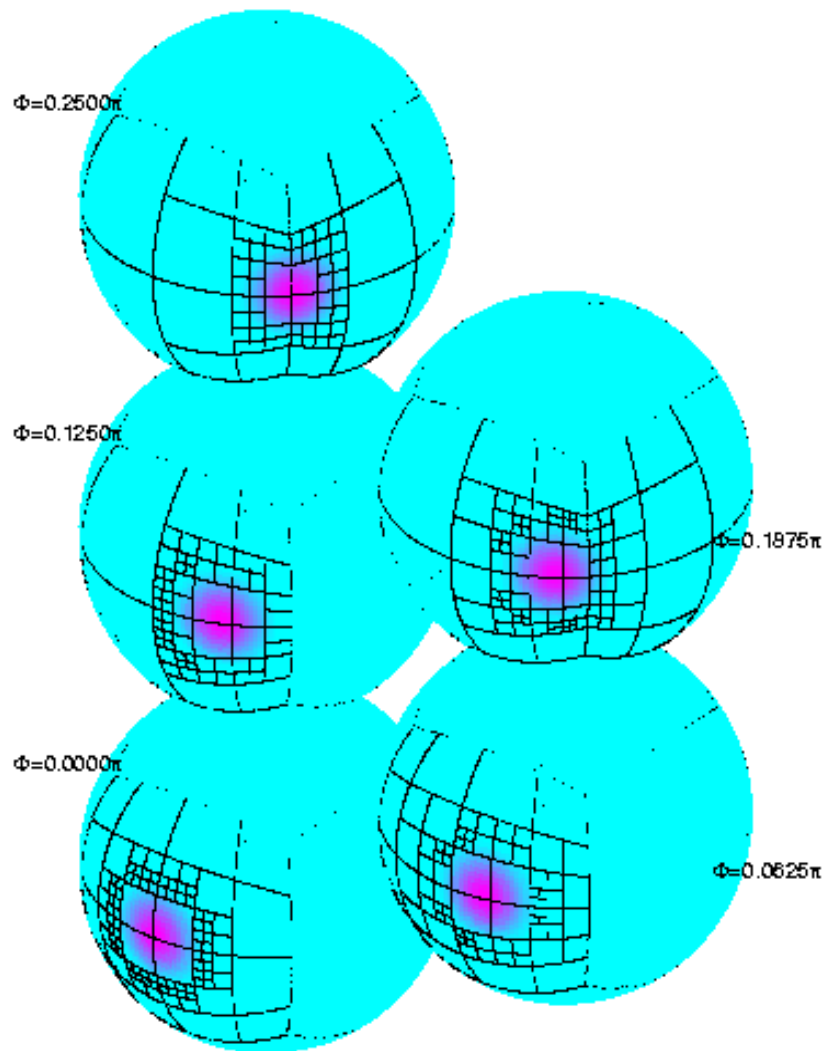
Figure 14: A cubed-sphere with embedded nests.
