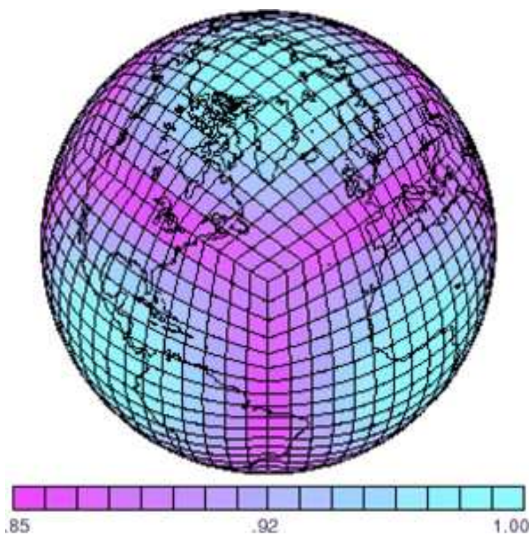
Figure 3: The cube-sphere grid, projecting the sphere onto the six faces of a cube. Polar singularities are avoided, at the expense of some grid distortion near the cube’s vertices.
