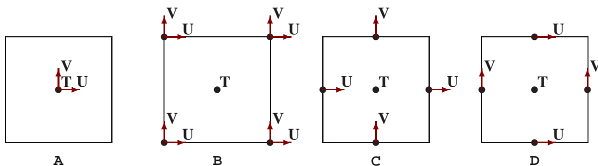
Figure 7: The Arakawa staggered grids.
