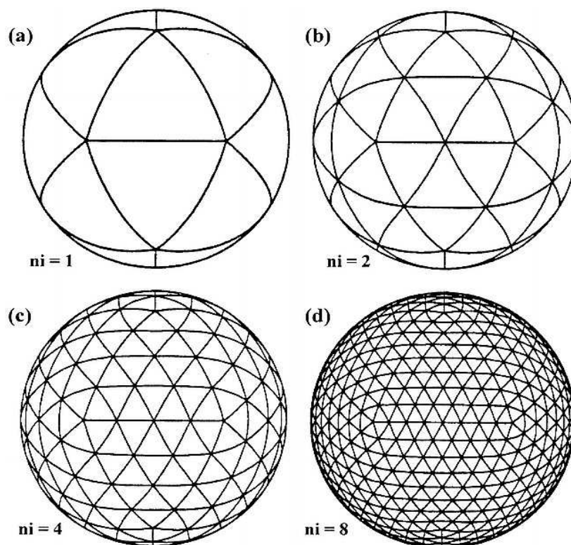
Figure 4: A structured triangular discretization of the sphere. Note that all vertices at any truncation level ni are also vertices at any higher level of truncation.
