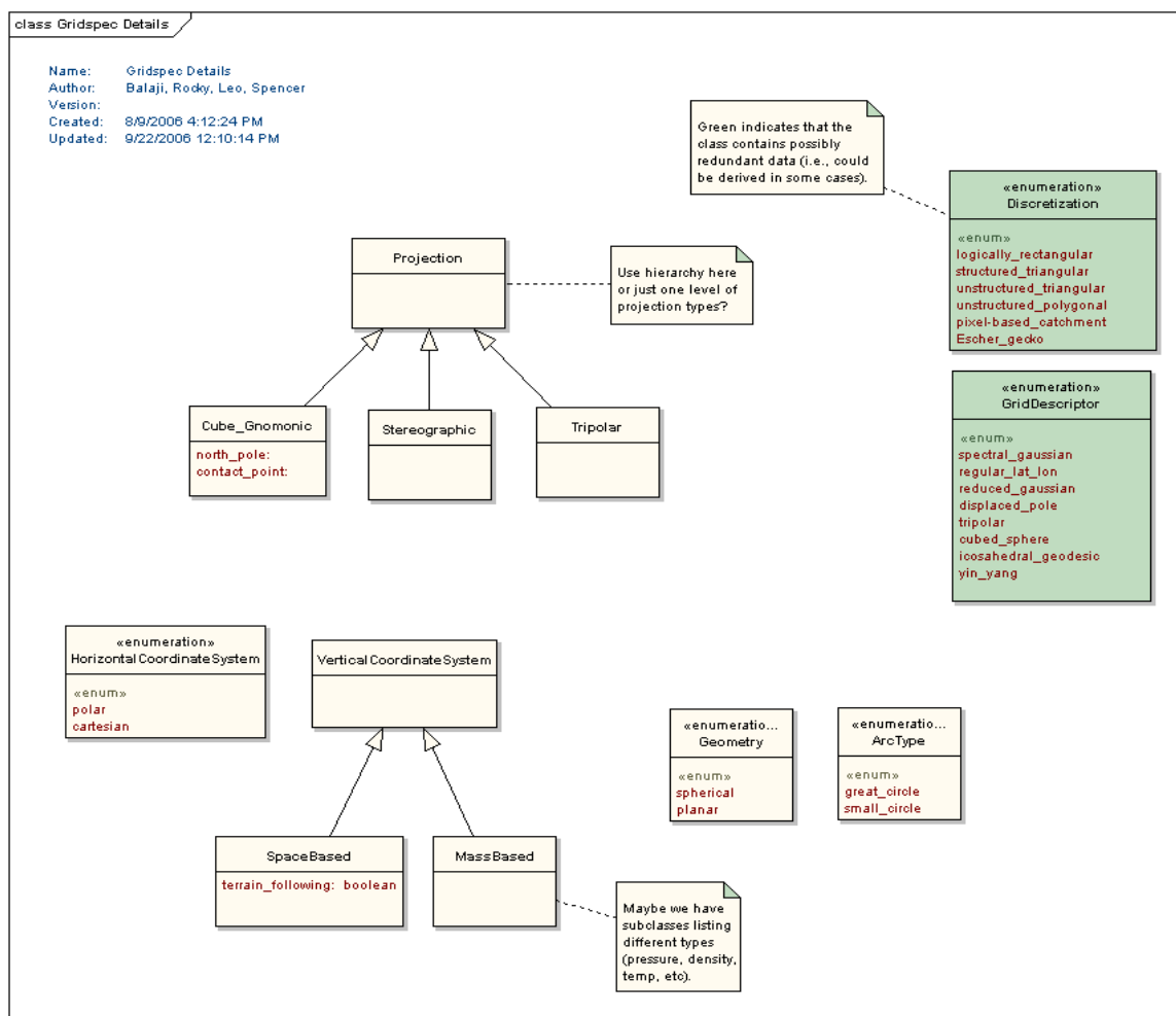
Figure 19: Semantics of grid specification. This UML diagram shows a vocabulary for describing grid coordinate systems, projections and discretizations. The proposal is that this semantic content uses a controlled, yet extensible, vocabulary maintained by the CF convention committees.
