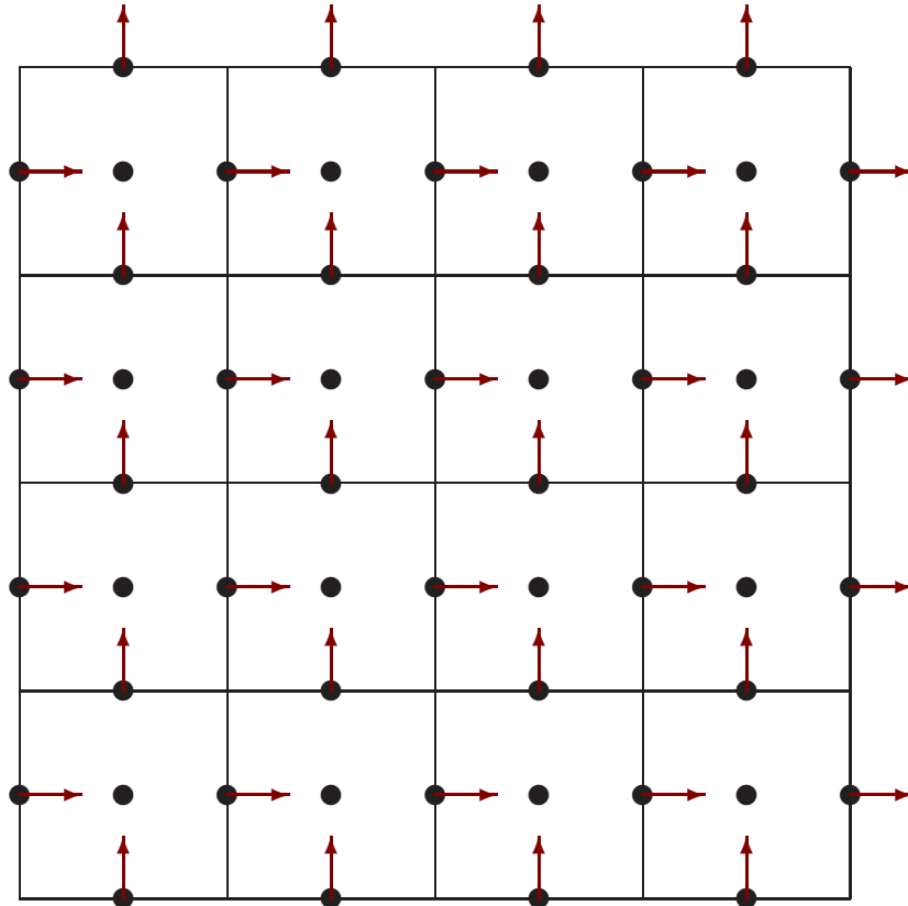
Figure 8: A 4 \times 4 (not 8 \times 8! ) Arakawa C-grid.
