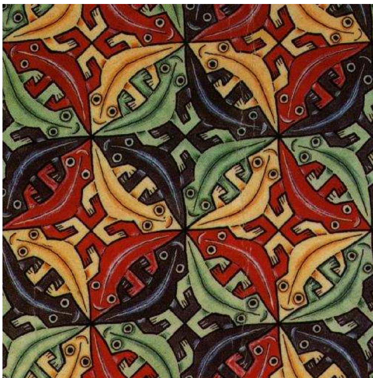
Figure 6: Another possible discretization of the plane.
