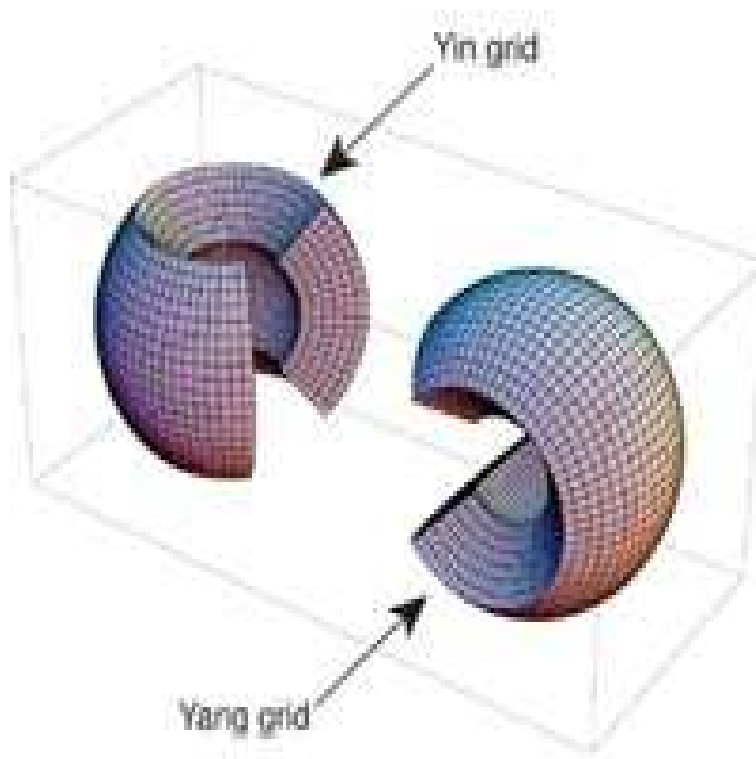
Figure 13: The yin-yang grid consists of two longitude-latitude bands with mutually orthogonal axes, and an overlap.
