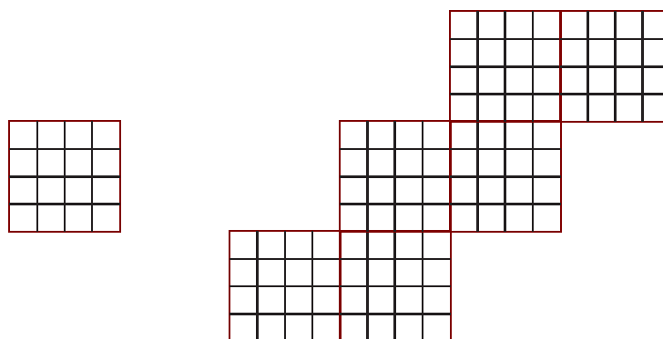
Figure 11: A grid tile: a quadrilateral grid shown in index space. A grid mosaic: a number of tiles sharing boundaries or contact regions.
