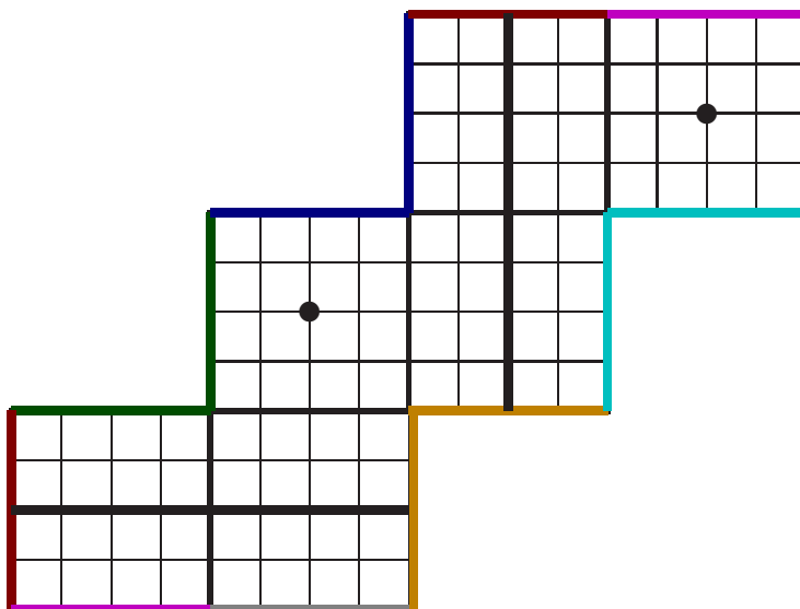
Figure 15: The cubed-sphere grid mosaic.
