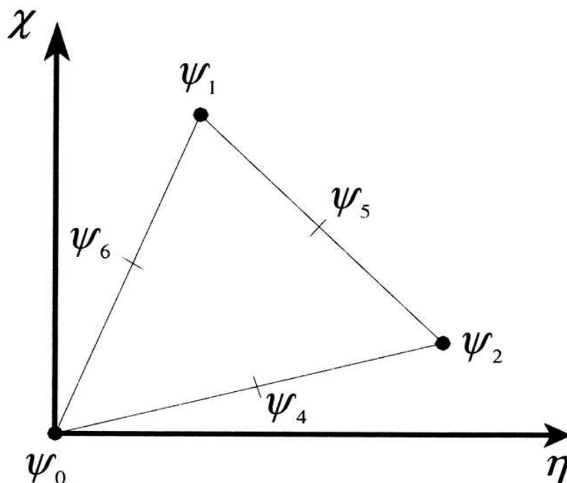
Figure 10: Vertex- and face-centered locations on a triangular grid. All of these quantities are needed for certain accurate interpolation algorithms on these grids. Further, different quantities may be placed on a different subset of points associated with this cell.
