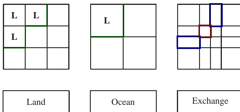
Figure 18: The mask problem. The land and atmosphere share the grid on the left, and their discretization of the land-sea mask is different from the ocean model, in the middle. The exchange grid, right, is where these may be reconciled: the red “orphan” cell is assigned (arbitrarily) to the land, and the land cell areas “clipped” to remove the doubly-owned blue cells.
