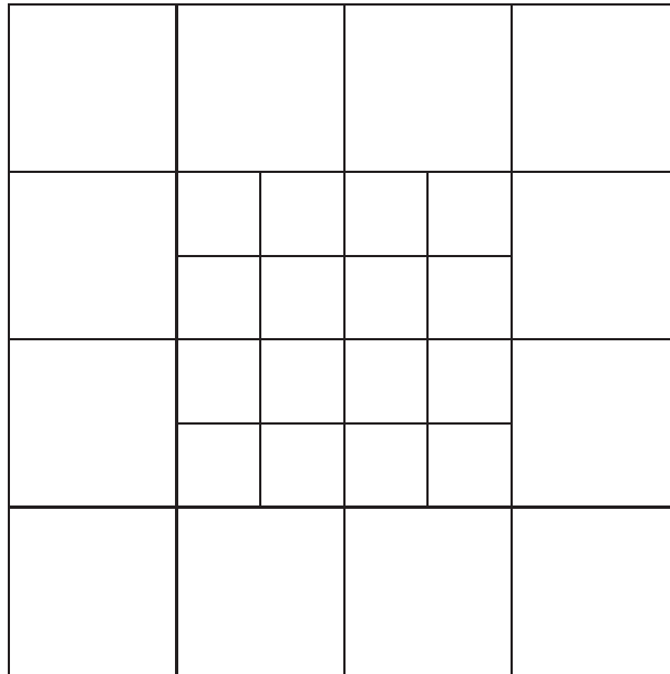
Figure 9: Nested grids with integer refinement: an inner 4 \times 4 grid at twice the resolution is nested within the coarse 4 \times 4 grid.
